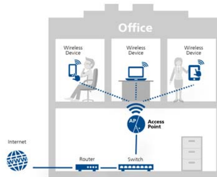
Abb. 2: WLAN-Access-Point
